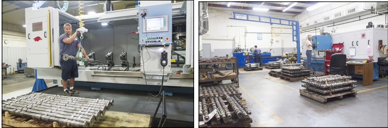
Left: Large CNC Camshaft Grinder for camshafts up to 100" in length. Right: Hillcrest Camshaft Production Grinding for the Over-the-Road Truck Engines.
